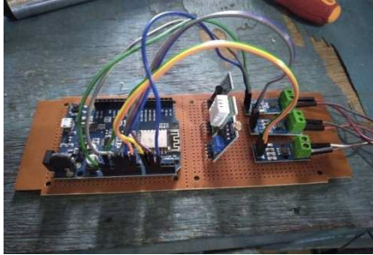
Fig. 5 The results of the installation of current sensors, light sensors, temperature sensors and thermal sensors
